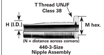
440-3-Size Nipple Assembly
