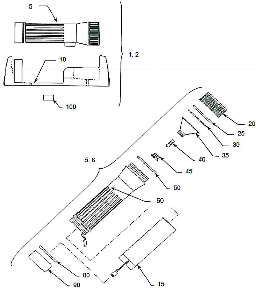
Figure 1 Model EF-2C Rechargeable Flashlight System
